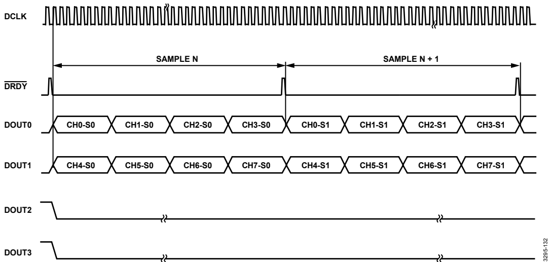
Figure 118. FORMAT0 = 0, FORMAT1 = 1 —Channel 0 to Channel 3 Share DOUT0 , and Channel 4 to Channel 7 Share DOUT1 (S0 Means Sample 0 and S1 Means Sample 1)
