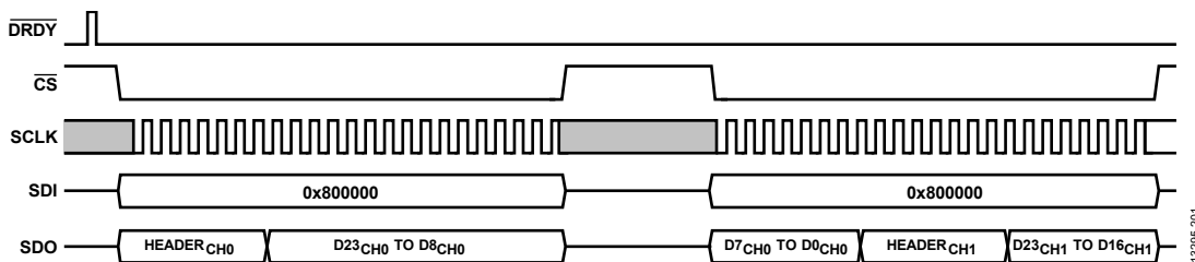
Figure 104. SPI Used to Read Back the Σ-Δ ADC Data, in 24-Bit Frames
