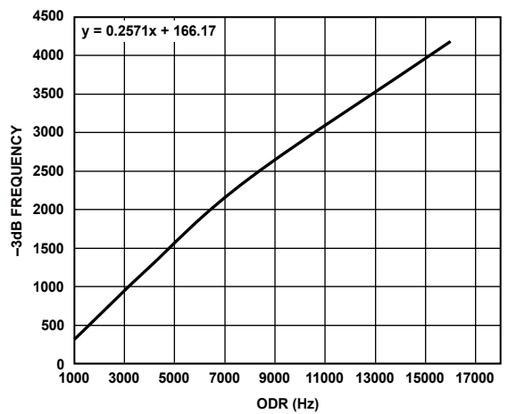
Figure 111. -3 dB Correction Factor, HR Mode
