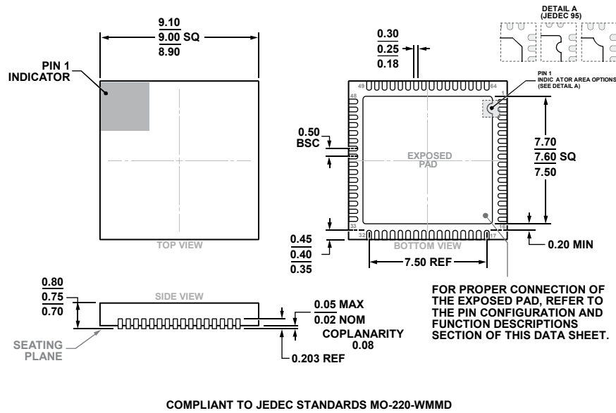
Figure 123. 64-Lead Lead Frame Chip Scale Package [LFCSP] 9 mm × 9 mm Body and 0.75 mm Package Height (CP-64-15) Dimensions shown in millimeters
