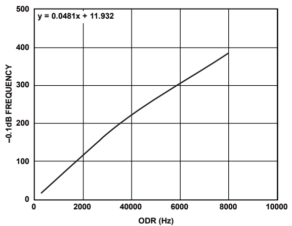
Figure 112. -0.1 dB Correction Factor, LP Mode
