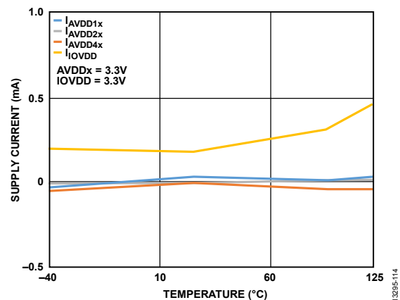
Figure 96. Shutdown Current
