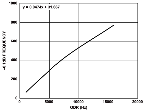
Figure 110. -0.1 dB Correction Factor, HR Mode
