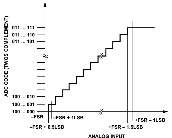
Figure 90. Transfer Function
