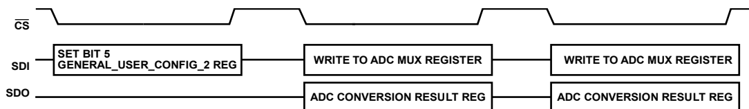
Figure 105. Configuring the AD7779 to Operate the SPI to Read from the SAR ADC
