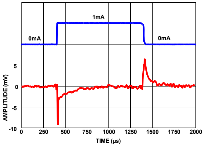
FIGURE 129. LOAD TRANSIENT RESPONSE AT 1mA LOAD @1μF
