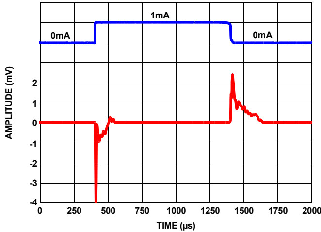
FIGURE 10. LOAD TRANSIENT RESPONSE AT 1mA LOAD @1μF
