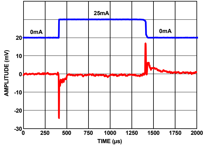
FIGURE 43. LOAD TRANSIENT RESPONSE AT 25mA LOAD @1μF
