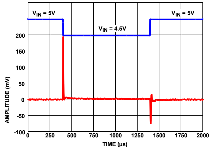
FIGURE 125. LINE TRANSIENT RESPONSE WITH 0.1µF LOAD
