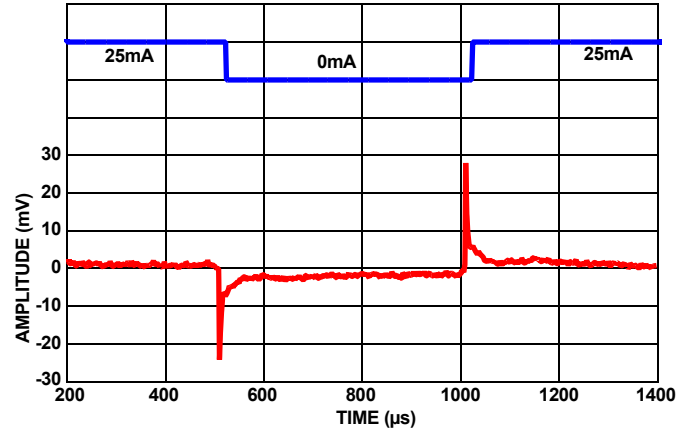
FIGURE 94. LOAD TRANSIENT RESPONSE AT 25mA LOAD @1μF
