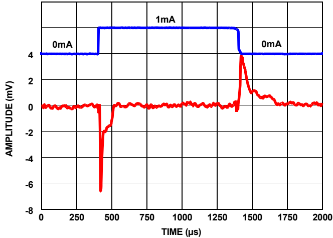
FIGURE 78. LOAD TRANSIENT RESPONSE AT 1mA LOAD @1μF
