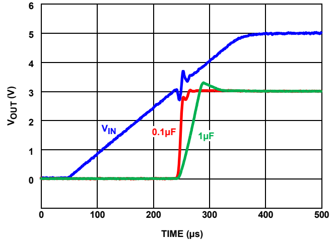
FIGURE 96. TURN-ON TIME
