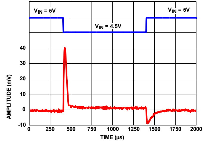
FIGURE 126. LINE TRANSIENT RESPONSE WITH 10µF LOAD
