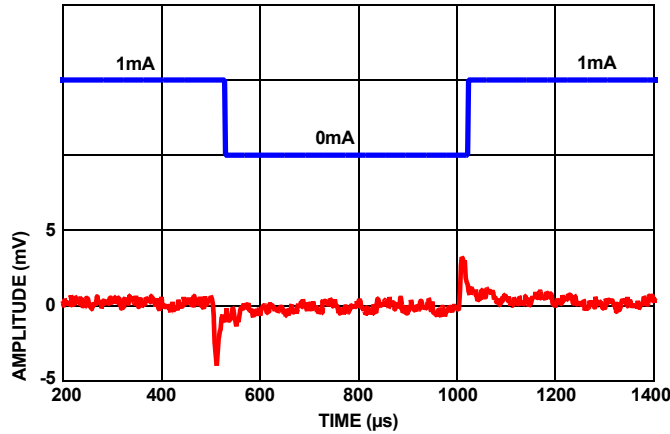
FIGURE 95. LOAD TRANSIENT RESPONSE AT 1mA LOAD @1μF
