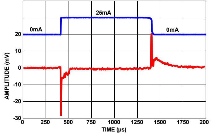
FIGURE 77. LOAD TRANSIENT RESPONSE AT 25mA LOAD @1μF
