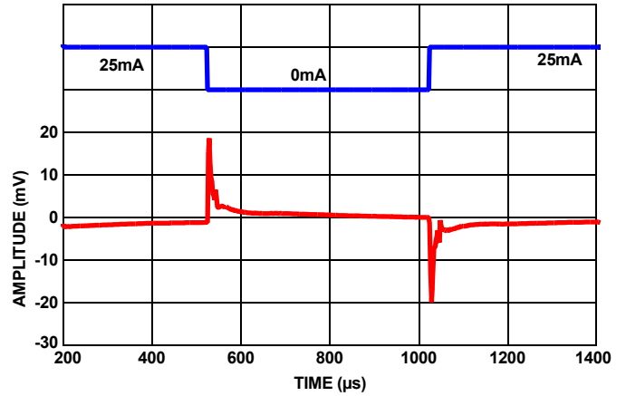
FIGURE 111. LOAD TRANSIENT RESPONSE AT 25mA LOAD @1μF
