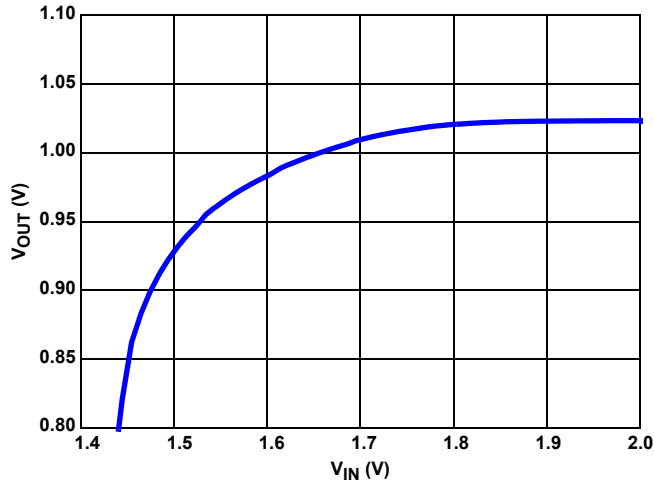
FIGURE 14. DROPOUT (10mA SOURCED LOAD)
