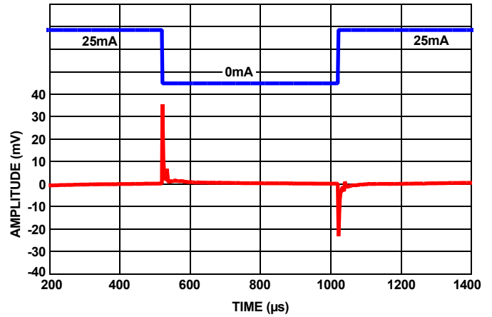
FIGURE 60. LOAD TRANSIENT RESPONSE AT 25mA LOAD @1 \mu F
