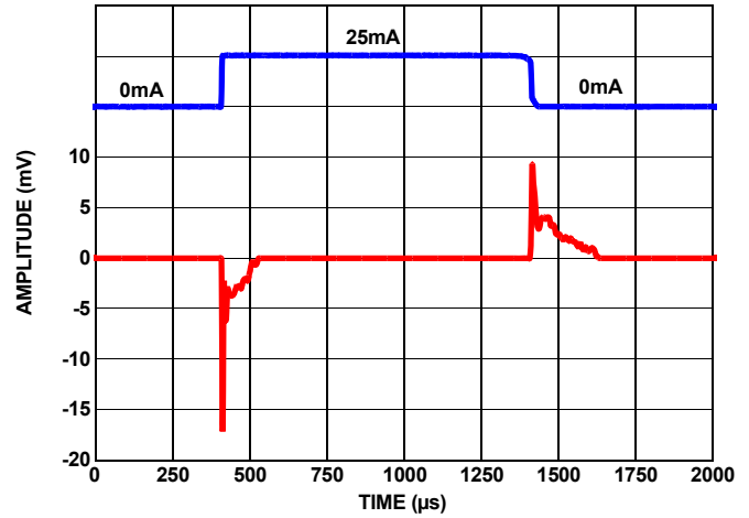
FIGURE 9. LOAD TRANSIENT RESPONSE AT 25mA LOAD @1μF
