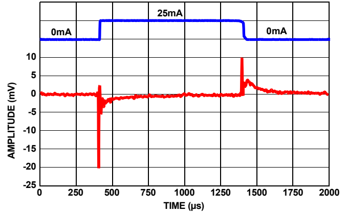
FIGURE 26. LOAD TRANSIENT RESPONSE AT 25mA LOAD @1μF
