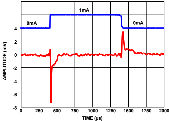
FIGURE 44. LOAD TRANSIENT RESPONSE AT 1mA LOAD @1μF
