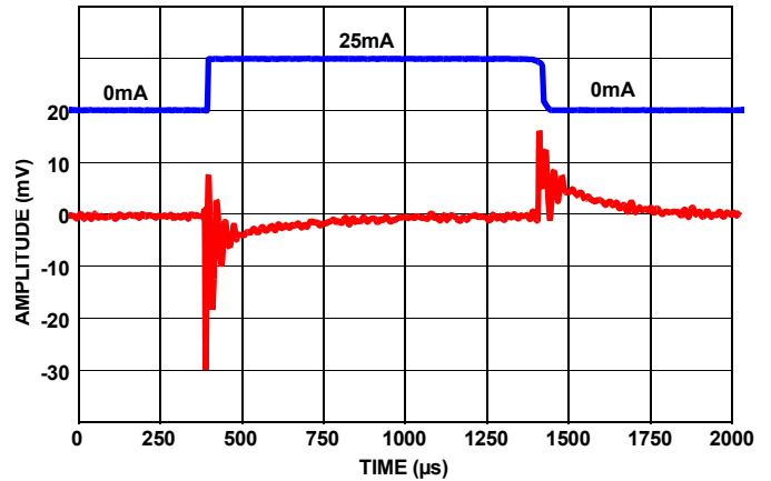
FIGURE 128. LOAD TRANSIENT RESPONSE AT 25mA LOAD @1μF
