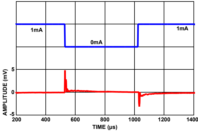
FIGURE 61. LOAD TRANSIENT RESPONSE AT 1mA LOAD @1 \mu F
