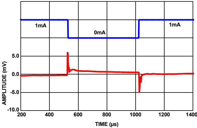
FIGURE 112. LOAD TRANSIENT RESPONSE AT 1mA LOAD @1μF
