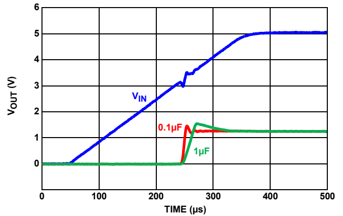
FIGURE 28. TURN-ON TIME
