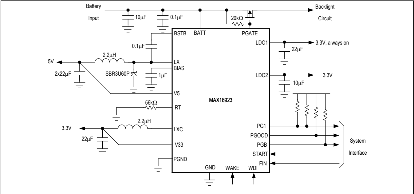
MAX16923A - HV Buck Operating at 2MHz
